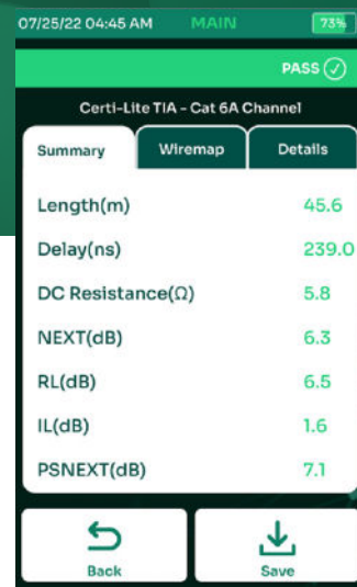
Figure 4 - Certi-Lite Autotest result can be obtained with Remote IDs.
